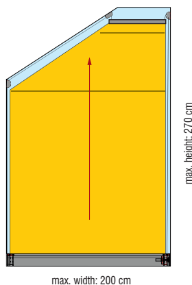
UNO 95.2-S (Slope)
